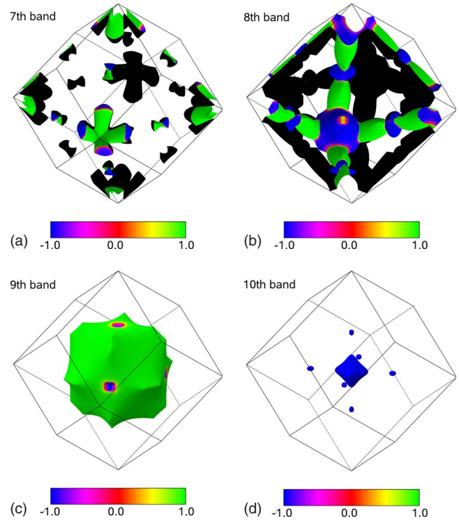
FIG. 5. (Color online) Calculated relativistic Fermi surface for the bands 7–10 of bcc Fe. The expectation values of the \hat{\beta}\sigma_z operator are given as color code.
