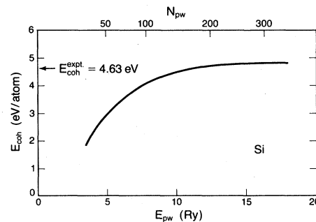
FIG. 3. Convergence test of the calculated cohesive energy ( E_{\text{coh}} ) of Si with respect to the kinetic-energy cutoff ( E_{\text{pw}} ) of the plane-wave basis set ( N_{\text{pw}} is the approximate number of the plane waves in the basis set).
