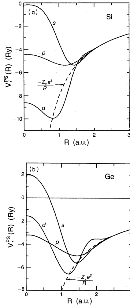
FIG. 1. Ab initio core pseudopotentials of (a) Si and (b) Ge generated using the reference valence configuration of s^2 p^{0.5} d^{0.5} . The letters s , p , and d denote the non-local pseudopotential for angular momenta l=0 , 1, and 2, respectively. Dashed line denotes the Coulomb potential of a (fictitious) pointlike atomic core.
