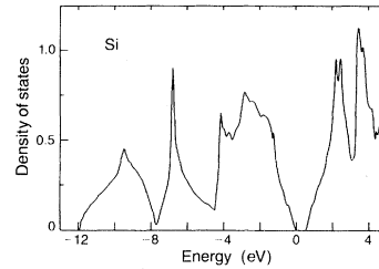
FIG. 17. Density of states of Si in units of state/eV atom. Energies are measured from the valence-band maximum.
