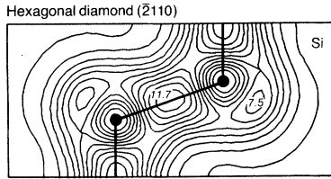
FIG. 7. Contour plot of the (valence) charge density in the (\bar{2}110) plane of the hexagonal diamond phase of Si at \Omega_{\text{expt}} (conventions of Fig. 4).
