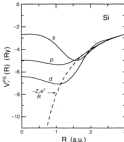
FIG. 19. Ab initio pseudopotential of Si generated using 1.35, 1.56, and 1.56 a.u. for r_c values of s , p , and d components.
