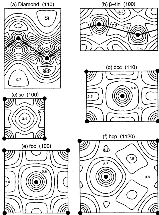
FIG. 8. Charge density contour plots of six phases of Si at 0.751\Omega_{\text{expt}} (conventions of Fig. 4).
