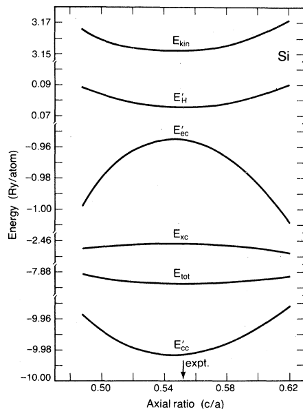
FIG. 12. Individual energy contributions of the \beta -tin phase of Si as a function of the axial ratio at a fixed atomic volume of 0.71\Omega_{\text{expt}} . (The contribution E'_{ec} has a constant 2.285 subtracted out.)
