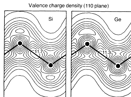
FIG. 4. Contour plots of the valence charge density in the (110) plane of the cubic diamond (CD) phase of Si and Ge at \Omega_{\text{expt}} (Ref. 31). Charge density is in units of electrons per atomic volume with a contour step of 1. The black dots denote the atomic positions and straight lines denote the atomic chains.
