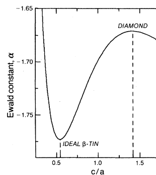
FIG. 13. Ewald constant of the \beta -tin phase as a function of axial ratio ( c/a ).
