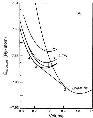
FIG. 11. Total-energy curves of the diamond phase and the \beta -tin phases with axial ratios (i) 0.552, (ii) 0.621, (iii) 0.488, and (iv) 0.458 as a function of the atomic volume normalized to \Omega_{\text{expt}} . Dashed line is the common tangent of the energy curves for the diamond phase and the \beta -tin phase (i).
