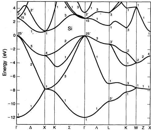
FIG. 15. Electronic structure of Si. Numbers refer to the conventional indices for symmetry group representations. Energies are measured from the valence-band maximum ( \Gamma_{25'} ).
