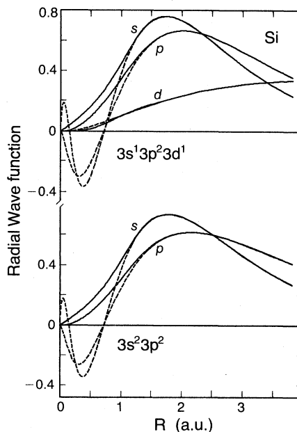
FIG. 2. Comparison between the pseudo (solid lines) and the corresponding all-electron (dashed lines) radial wave functions for the configurations 3s^2 3p^2 and 3s^1 3p^2 3d^1 of Si.
