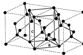
FIG. 10. Ball-and-stick model for the diamond crystal structure. Dashed lines denote the cubic unit cells and solid lines denote the tetragonal unit cell.
