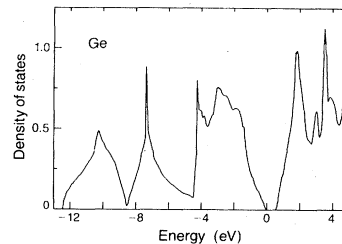
FIG. 18. Density of states of Ge (conventions of Fig. 17).
