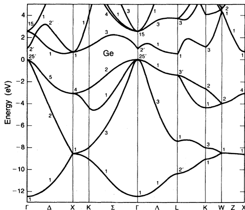
FIG. 16. Electronic structure of Ge (conventions of Fig. 15).
