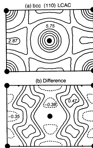
FIG. 9. (a) Contour plot of the charge density of the bcc phase of Si at 0.751\Omega_{\text{expt}} constructed from a superposition of pseudoatomic charge densities. (b) Contour plot of the difference between Figs. 8(d) and 9(a) (conventions of Fig. 4).
