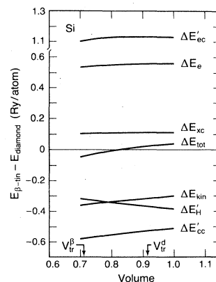
FIG. 14. Differences between various contributions to the total energy of the diamond phase and the \beta -tin phase ( c/a = 0.552 ) of Si as a function of atomic volume (normalized to \Omega_{\text{expt}} ).
