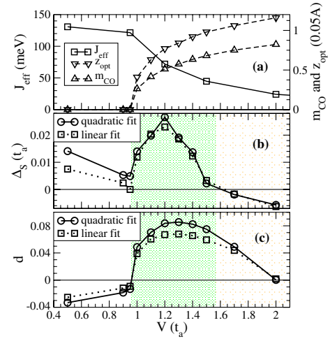
FIG. 3 (color online). Results for the EHM with coupling to the lattice, as a function of V . Extrapolated values of (a) the charge order parameter m_{CO} , (b) the spin gap \Delta_S , and (c) the dimerization d are illustrated for two coupled ladders ( t_{ab} = 0.17t_a ). The effective magnetic exchange constant J_{\text{eff}} [8] and the distortion z_{\text{opt}} [8] of an isolated ladder are also shown in (a). The three regimes discussed in the text are highlighted.
