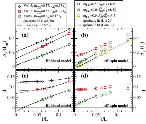
FIG. 2 (color online). Examples of finite-size extrapolations for (a), (b) the spin gap \Delta_S and (c), (d) the dimerization d of (a), (c) the Hubbard model and of (b), (d) the effective spin model. Linear and quadratic fits in 1/L are illustrated for charge-disordered states ( m_{CO} = 0 , circles) and SAF-ordered states ( m_{CO} > 0 ).
