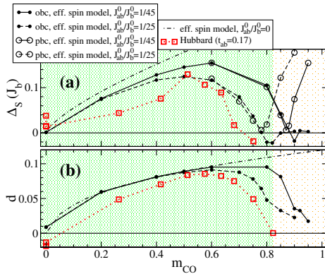
FIG. 4 (color online). Effective spin model. Quadratically extrapolated values ( L = \infty ) for (a) the spin gap \Delta_S and (b) the dimerization d , as a function of the charge order parameter m_{CO} . Calculations with OBC (black dots) and PBC (open circles) in the b direction are shown. For comparison the spin gap \Delta_S for the EHM is shown, in units of J_{\text{eff}} [Fig. 3(a)].
