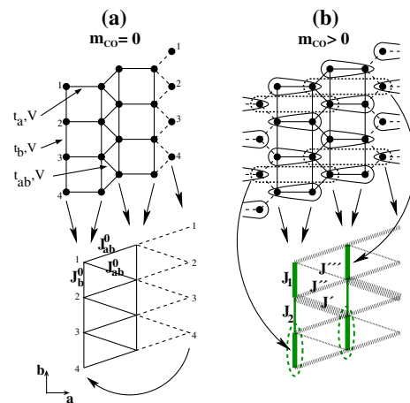
FIG. 1 (color online). Quarter-filled coupled ladders in \text{NaV}_2\text{O}_5 . The mapping of a rung (top) onto an effective spin site (bottom) is illustrated for (a) a charge-disordered and (b) a SAF-ordered regime. The shifted periodic boundary conditions in the a direction are indicated by numbers which identify identical sites. The proposed singlet formation for \text{NaV}_2\text{O}_5 is depicted by dashed ellipses in the effective spin model [(b), bottom].
